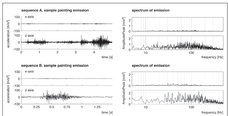
Figure 4 Emission measured on the canvas: acceleration and frequency spectrum
