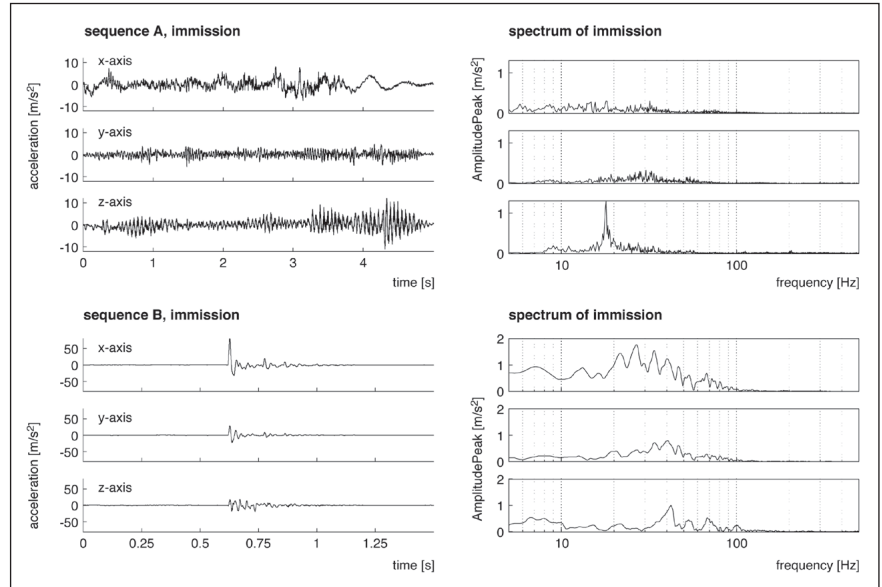
Figure 3 Immission measured on the frame: acceleration and frequency spectrum
